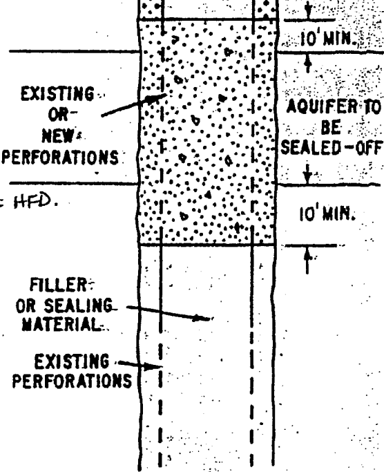
B. DEEP WELL WITH AQUIFER SEAL
