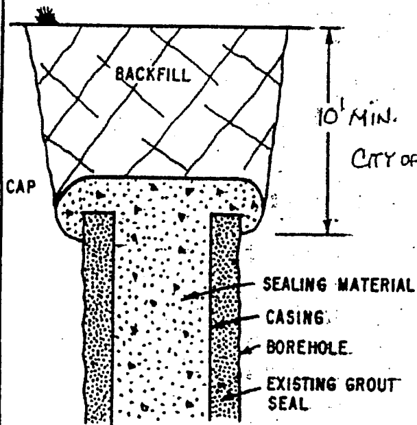
C. UPPER SEALING FEATURES URBAN AREA WELL
