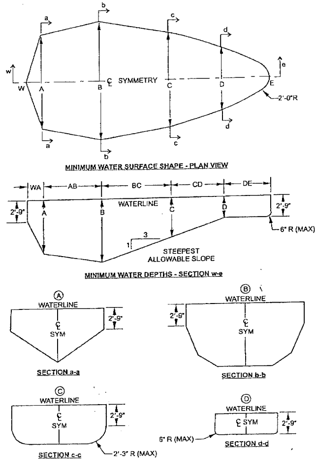
FIGURE 804.1 MINIMUM DIVING WATER ENVELOPE
